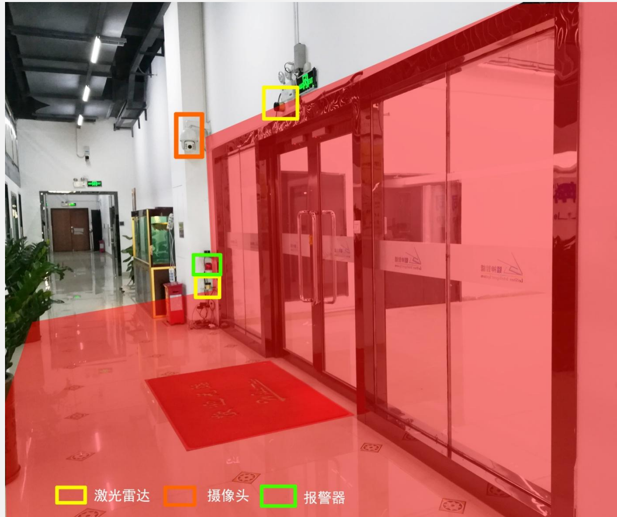
边界安防：激光雷达与摄像头联动
